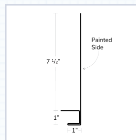
Overhead Door Trim
