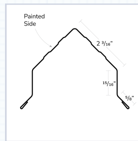
Small Corners Rake
