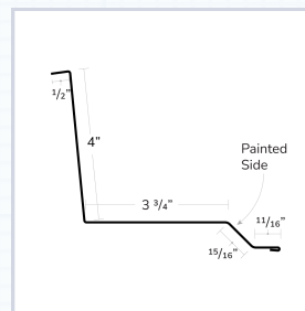
Chimney Flashing
