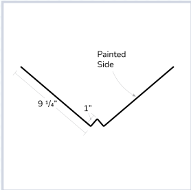
Track Cover
