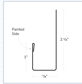
J-Channel
