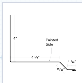
Sidewall Flashing
