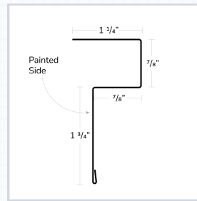
Overhang Trim
