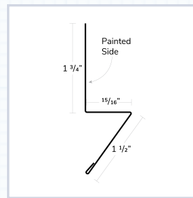
Rat Guard
