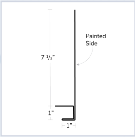
Overhead Door Trim
