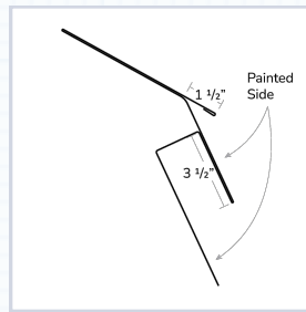
S.S. Gambrel
