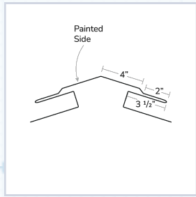
S.S. Ridgcap
