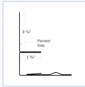
S.S. Sidewall
